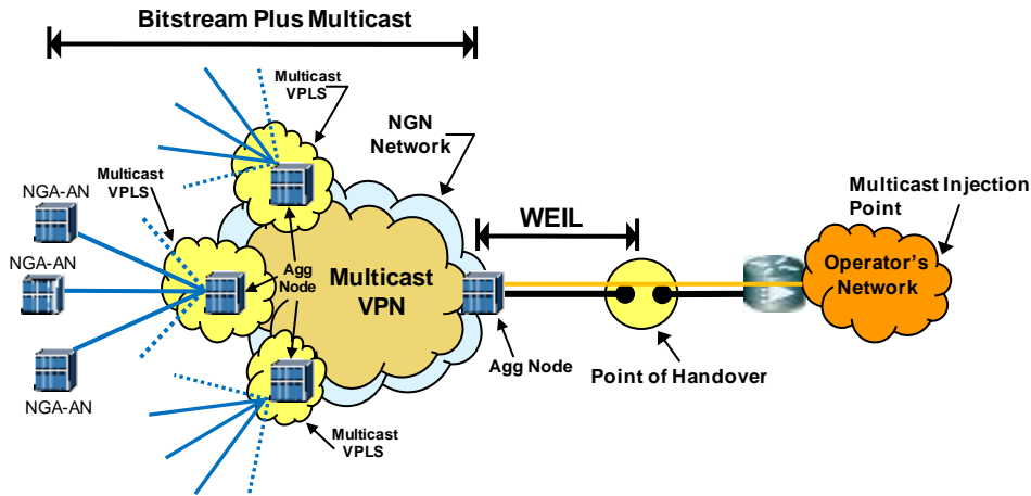
Figure 7: Bitstream Plus Multicast Service
