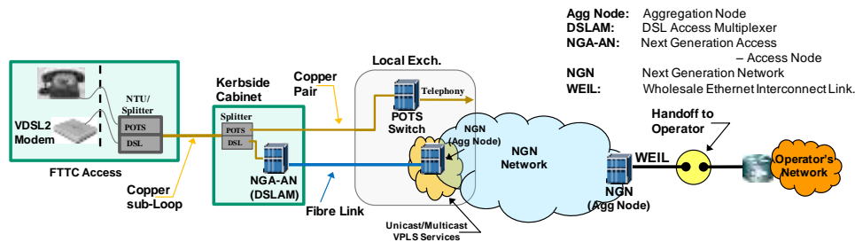
Flautre 16: FTTC Bitstream Plus POTS-Based
