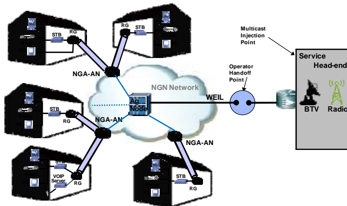
Figure 6: Multicast Principles
