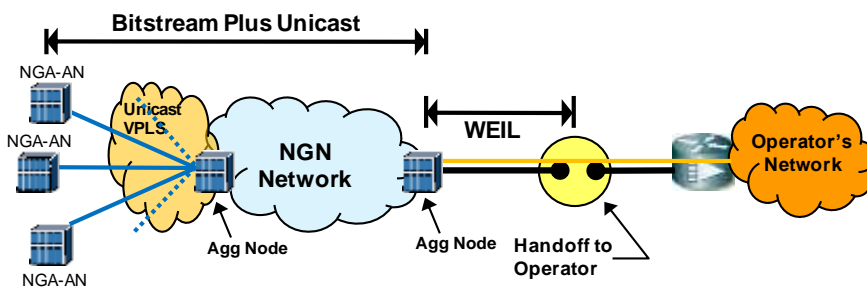
Figure 5: Bitstream Plus Unicast Service
