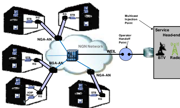
Figure 6: Multicast Principles
