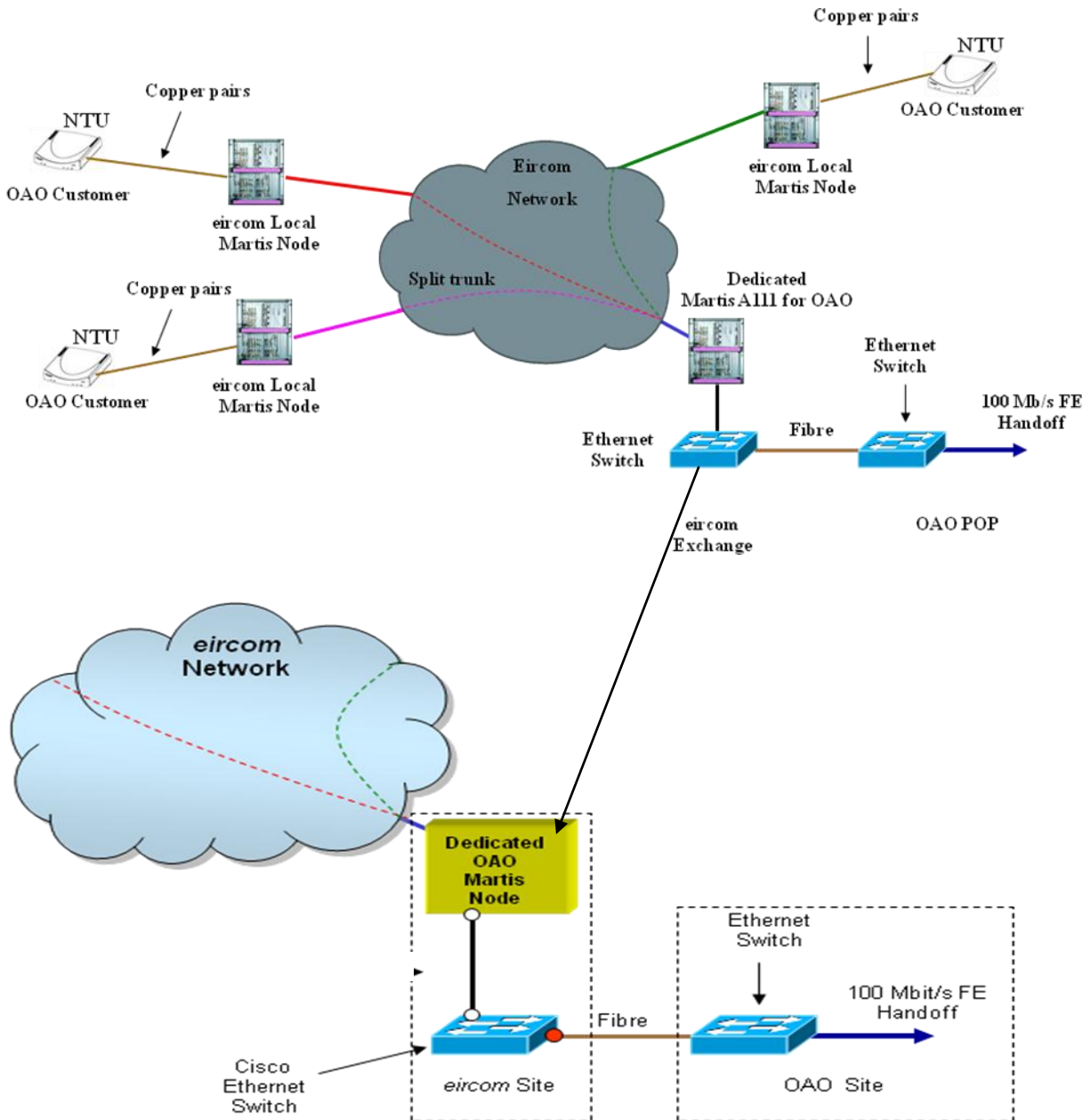
Figure 7: Operator Site handoff (Contended)
