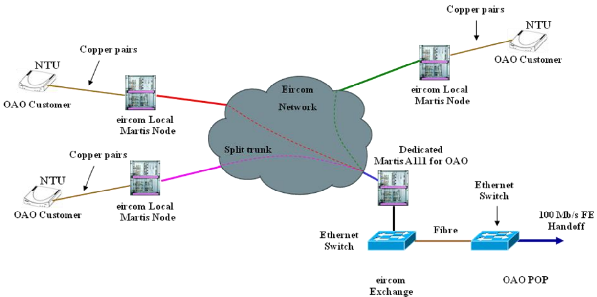
Figure 1: Operator Site handoff (Uncontended)
