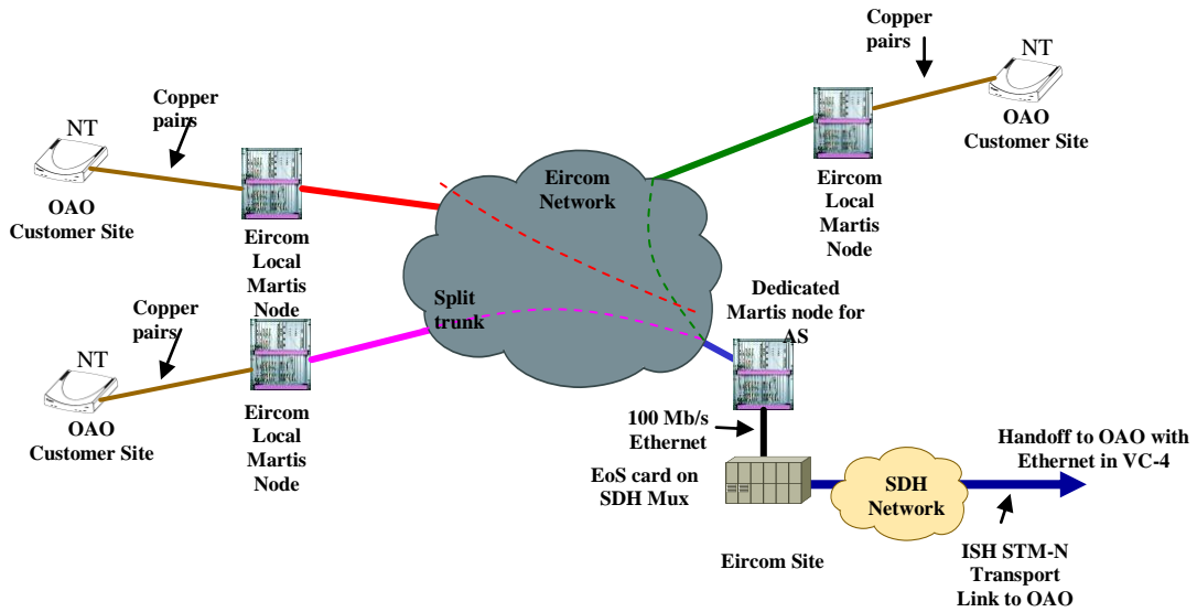
Figure 4: Ethernet over SDH In Span Handoff (Uncontended)
