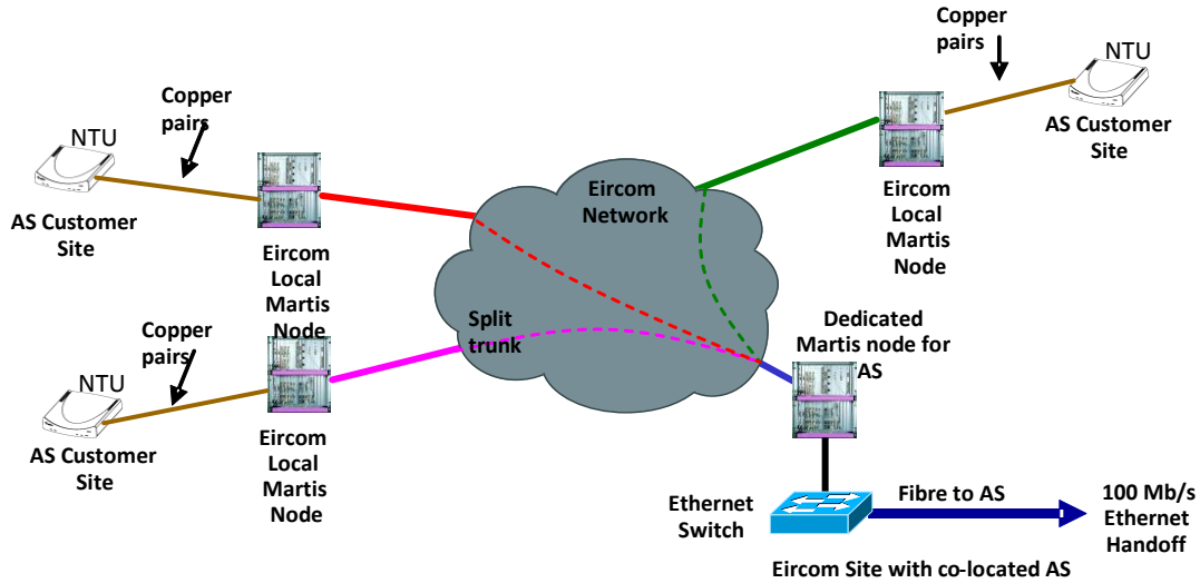
Figure 5: In Building Handover (Uncontended)
