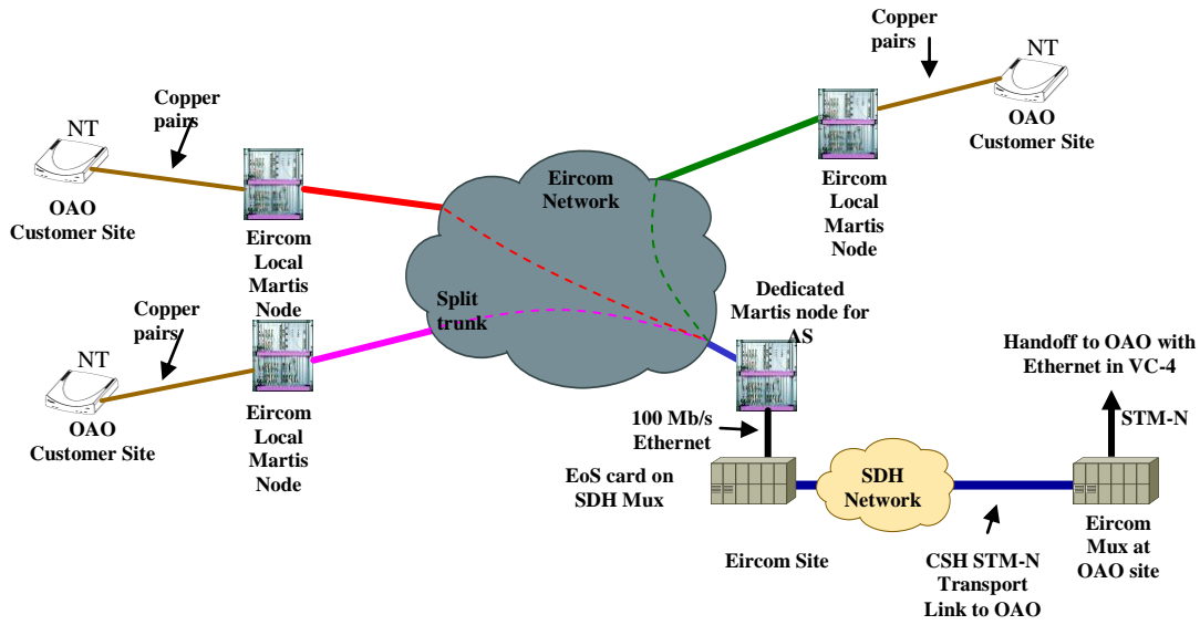
Figure 8: Handoff over SDH (Contended)
