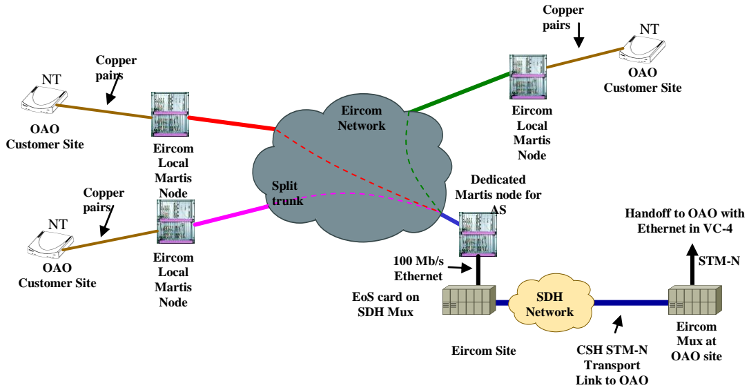
Figure 3: Ethernet over SDH Operator Site Handoff (Uncontended)
