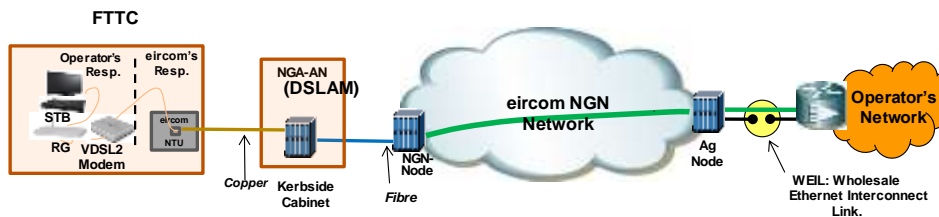
Figure 15: FTTC Standalone Bitstream Plus
