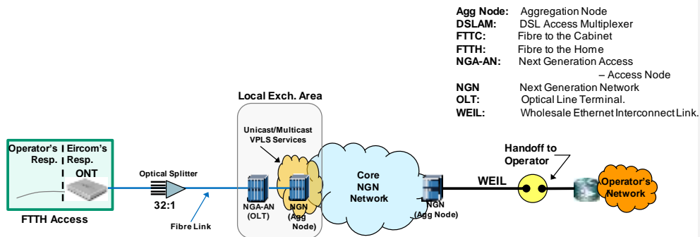
Figure 12: FTTH Bitstream Plus Standalone
