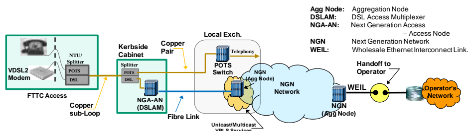
Figure 16: FTTC Bitstream Plus POTS-Based
