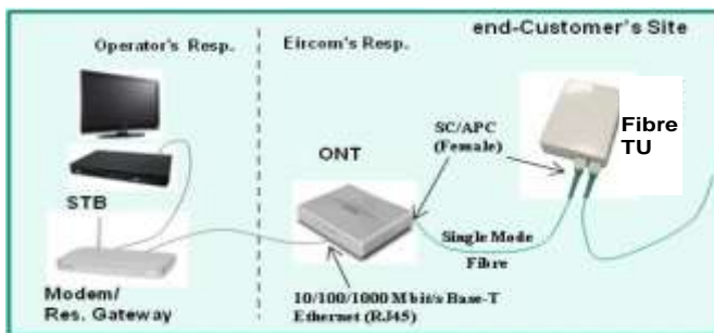
Figure 14: Fibre STP for FTTH
