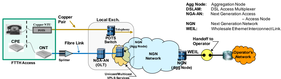
Figure 13: FTTH Bitstream Plus POTS-Based
